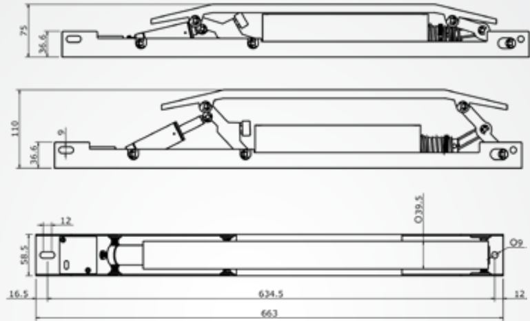
Lift Landing Door Retiring Cam (LDRC-M1)
