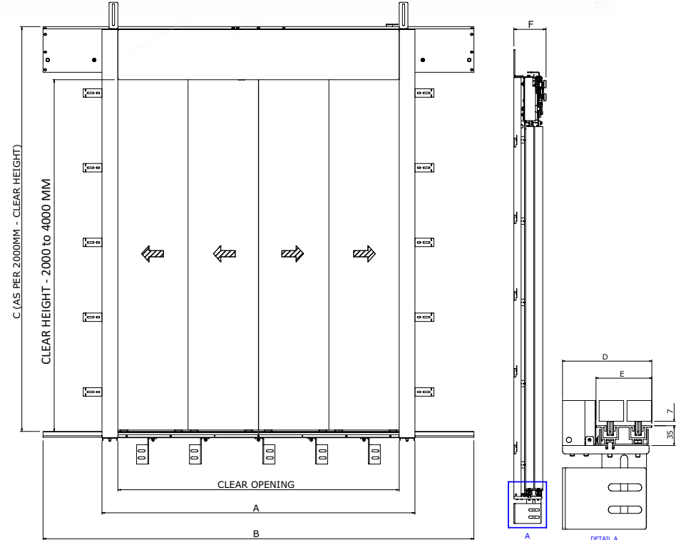
Clearing Opening of Autodoor for Landing
