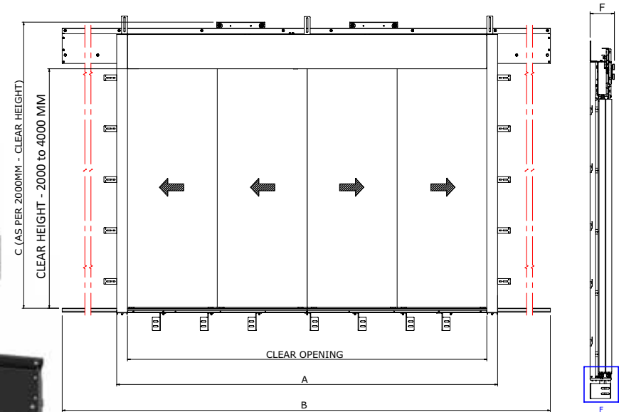
Clearing Opening of Autodoor for Landing
