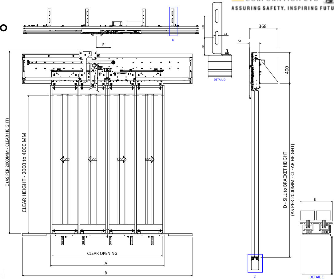
Clearing Opening of Autodoor for Car
