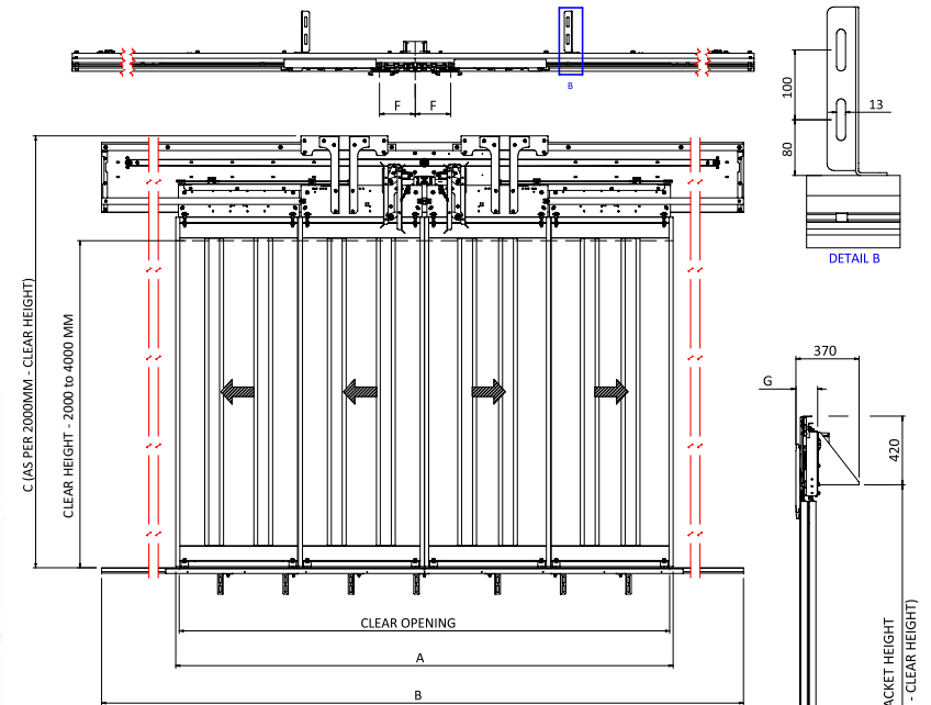
Clearing Opening of Autodoor for Car
