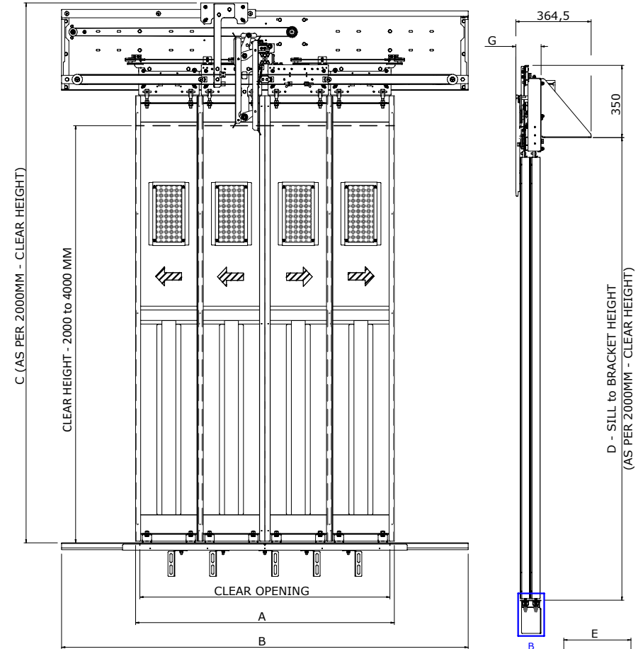
Clearing Opening of Autodoor for Car
