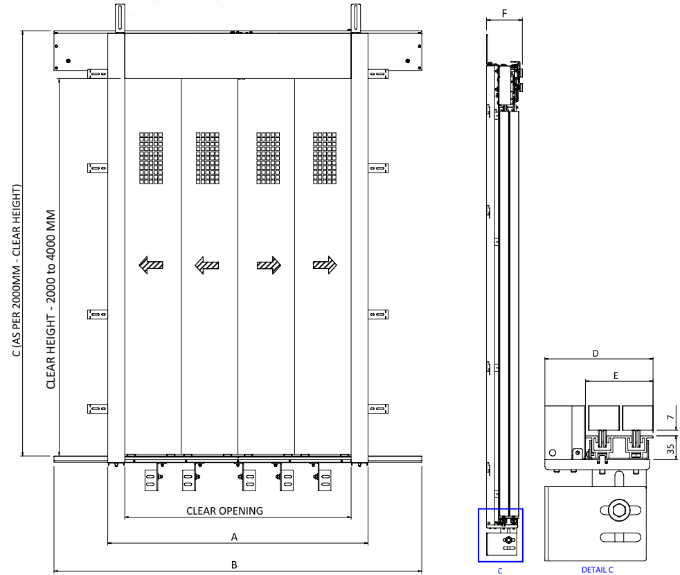
Clearing Opening of Autodoor for Landing
