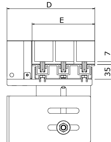
DETAIL D
